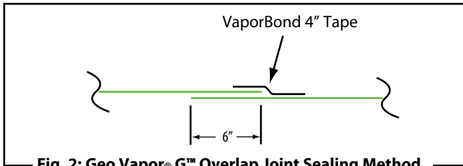
Fig. 2: Geo Vapor® G™ Overlap Joint Sealing Method
